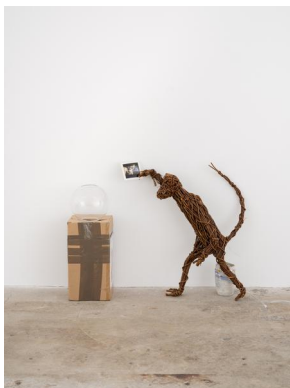
AES-RS4
